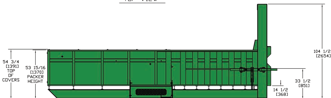
SIDE VIEW
