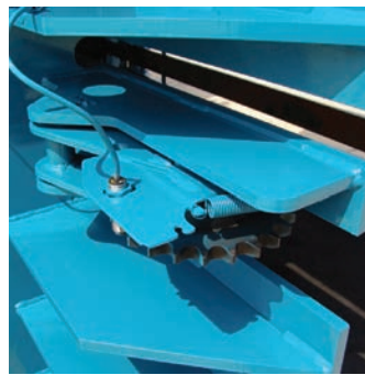
Spring-loaded counter wheel, located on the side of the baler, sends a digital reading to the operator interface.
