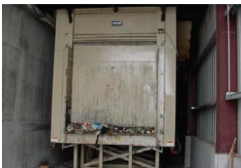
The BlokPak 3000 fits nicely into existing transfer stations with over-the-top feed systems such as this one located in Black Foot, ID.
